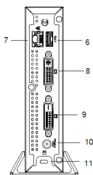
Rear View
